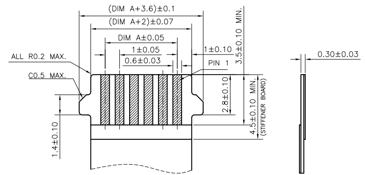
RECOMMENDED FPC/FFC DIMENSIONS GENERAL TOLERANCE ±0.05
